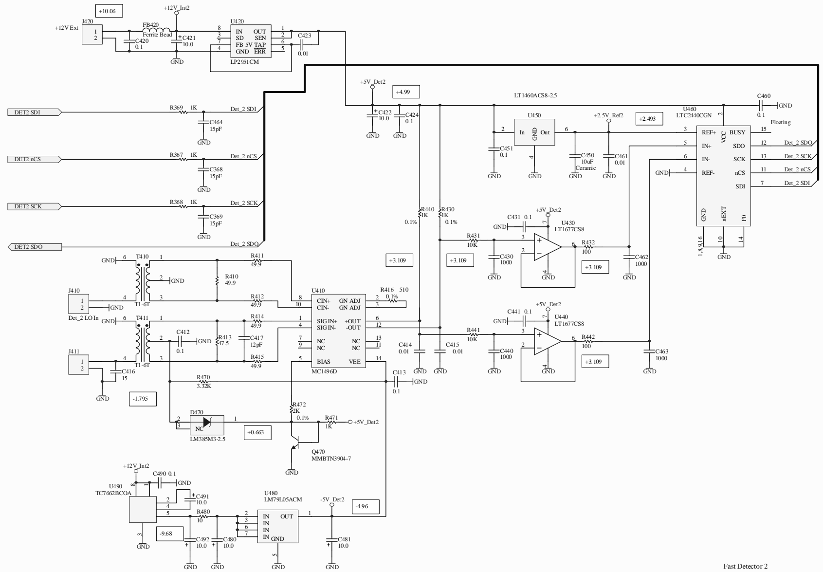
Fast Detector 2
